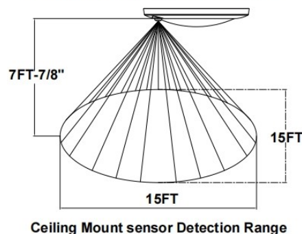
Ceiling Mount sensor Detection Range
