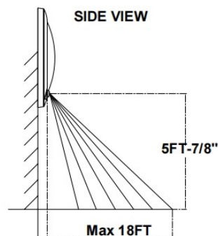
Wall Mount sensor Detection Range
