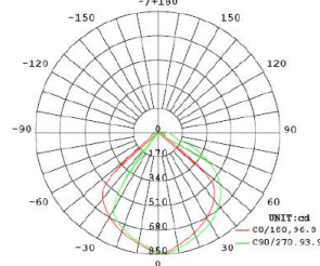
Luminous Intensity Distribution
