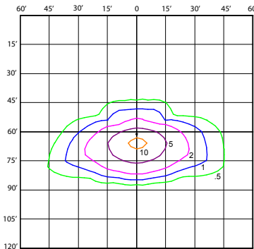
TYPE 3 - 60W 15' MOUNTING HEIGHT
