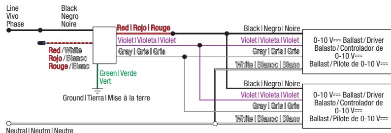
Image #49 — Dimmer with One Black Wire, Two Red Wires, One Violet Wire, and One Gray Wire in a Single Pole Application
