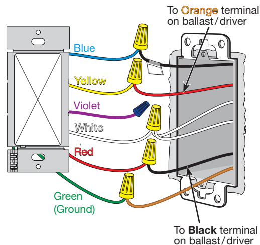
Image #42 — Dimmer with One Blue Wire, One Violet Wire, One Red Wire, One Yellow Wire and One White Wire in a Single Pole Application
