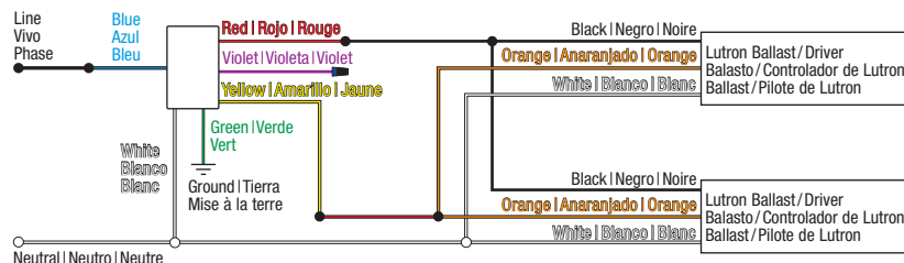
Image #42 — Dimmer with One Blue Wire, One Violet Wire, One Red Wire, One Yellow Wire and One White Wire in a Single Pole Application
