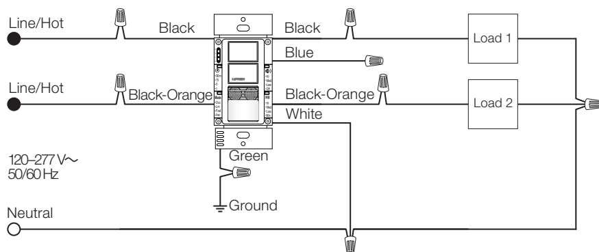
Single Pole, Two Breaker Feed Installation 1 (MS-A202)
