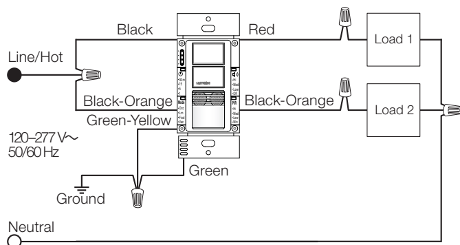
Single Pole, Single Breaker Feed Installation (MS-A202)
