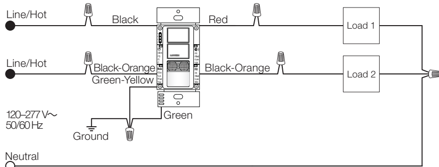
Single Pole, Two Breaker Feed Installation 1 (MS-A202)
