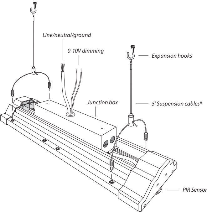
SUSPENSION MOUNTING TO ANCHORED HOOKS
