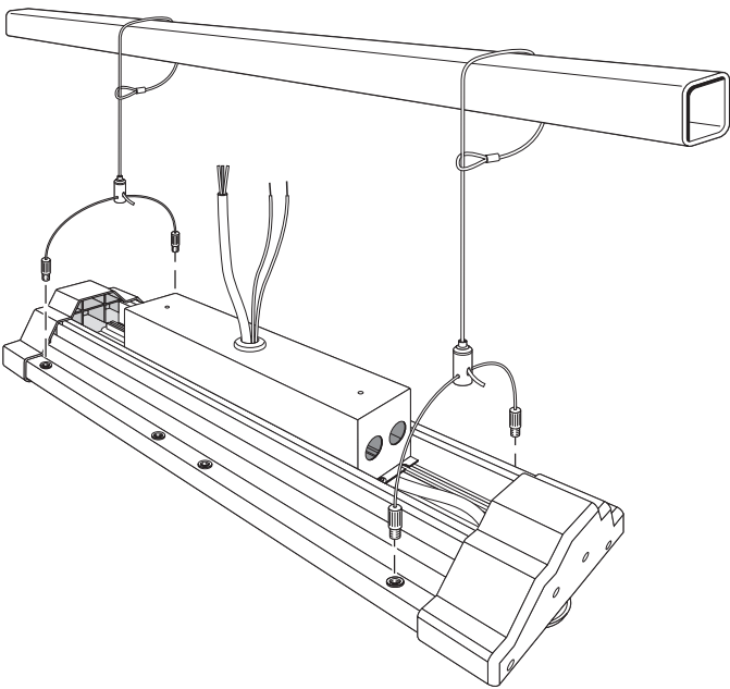
SUSPENSION MOUNTING TO BEAM
