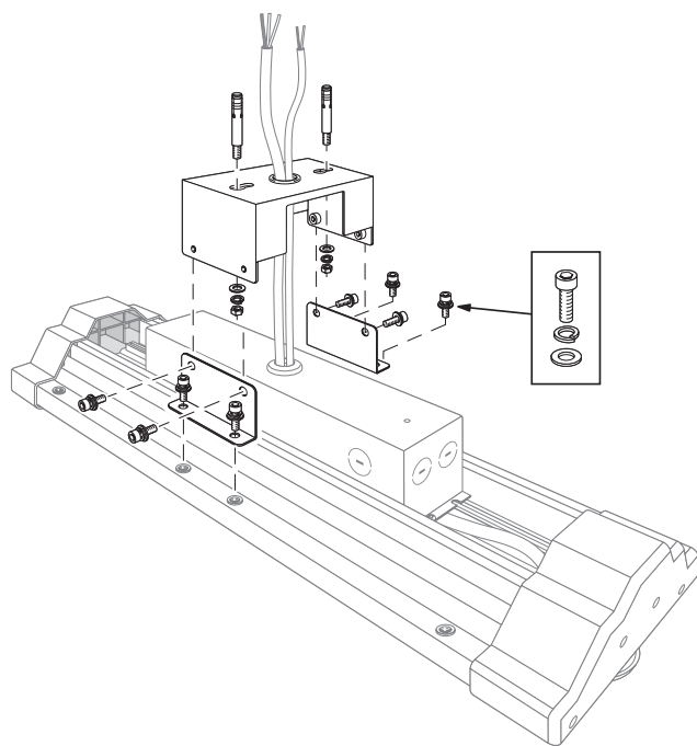
SURFACE MOUNTING*
