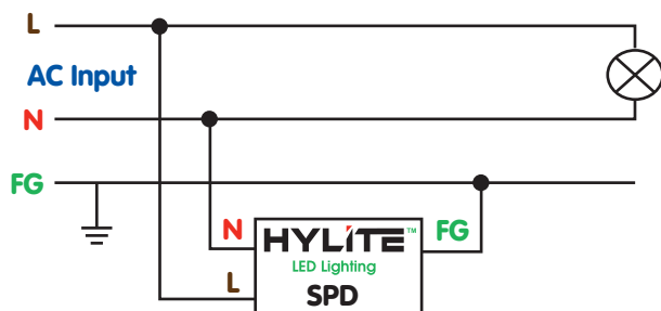
Wiring Diagram with External HyLite SPD, HL-SPD-20K
