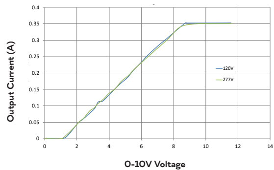
Dimming Curve
