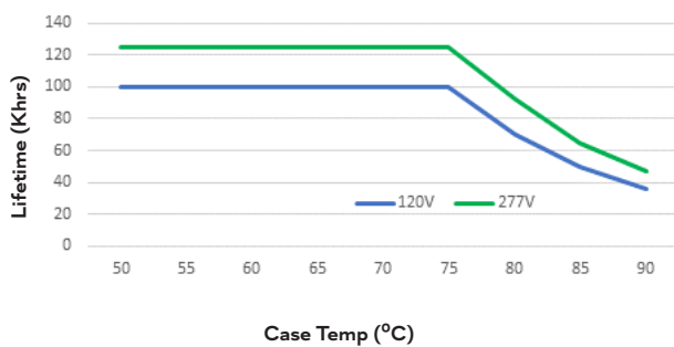
Lifetime vs. Case Temp
