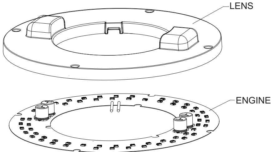
Exploded View
