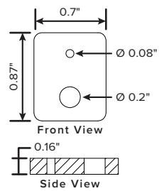
Hanger Block
