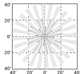
Zhaga Bluetooth® Sensor Coverage Top View
