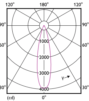
Light Distribution Diagram - 8.5PAR30L/COR/930/F25/D/P/ULW/T20 6/1FB
