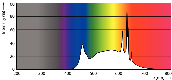
Spectral Power Distribution Colour - 13PAR38/COR/950/F40/DIM/P/ULW/T20 6/1FB
