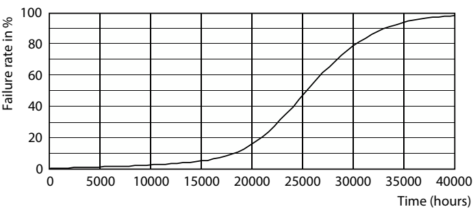
Life Expectancy Diagram - 13PAR38/COR/927/F40/DIM/P/ULW/T20 6/1FB
