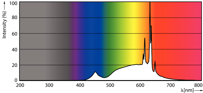
Spectral Power Distribution Colour - 13PAR38/COR/927/F25/DIM/P/ULW/T20 6/1FB
