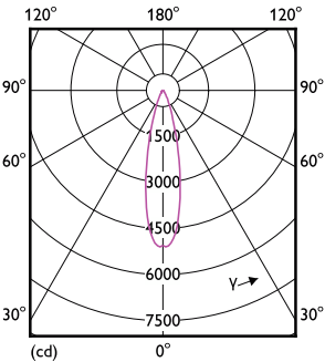
Light Distribution Diagram - 13PAR38/COR/927/F25/DIM/P/ULW/T20 6/1FB
