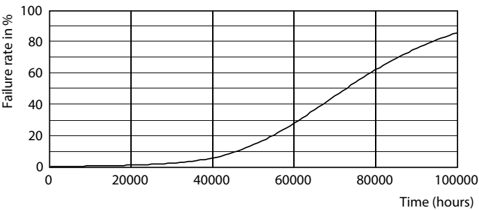
Life Expectancy Diagram - 10T8/COR/48-850/DF16/G/DIM UL-C 25/1
