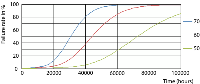
Life Expectancy Diagram - 10T8/COR/48-850/DF16/G/DIM UL-C 25/1
