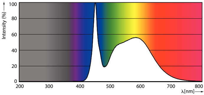
Spectral Power Distribution Colour - 115CC/LED/3CCT/LS EX39 BB 3/1
