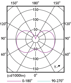
Light Distribution Diagram - 115CC/LED/3CCT/LS EX39 BB 3/1
