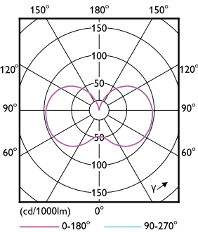
Light Distribution Diagram - 80CC/LED/3CCT/LS EX39 BB 3/1
