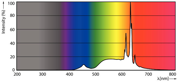
Spectral Power Distribution Colour - 5.5ST19/VIN/927/E26/CL/G/SP D 1PF T20
