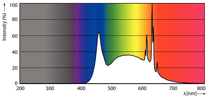
Spectral Power Distribution Colour - 15BR30/PER/950/P/E26/D/HO/T20 4/1PF
