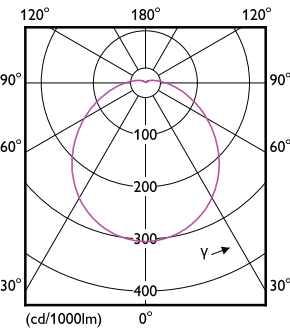
Light Distribution Diagram - 15BR30/PER/950/P/E26/D/HO/T20 4/1PF
