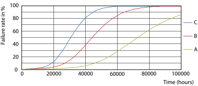
LEDtube_70K_FailureRate-LED
