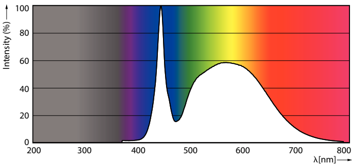
LEDtube MAS 14,5W G13 2100lm 850
