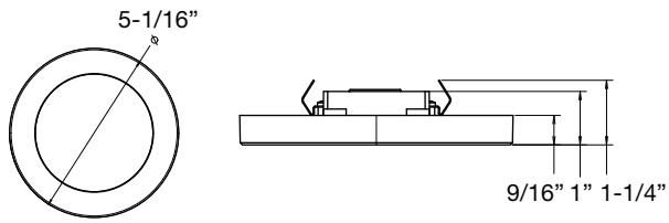
SLMFT5/9CCTS/DIM120V
