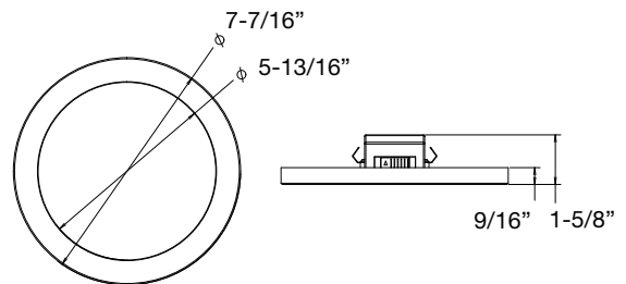
SLMFT7/9CCTS/DIM010UNV
