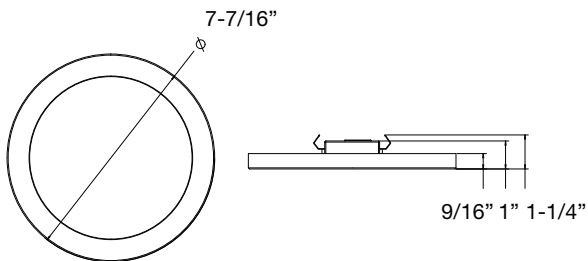
SLMFT7/9CCTS/DIM120V
