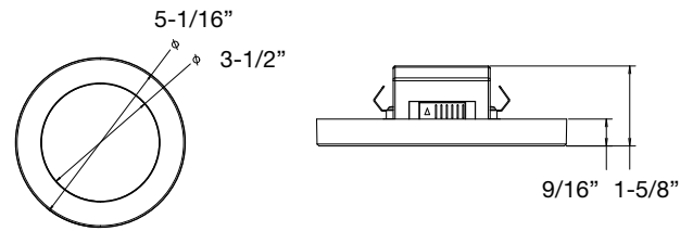
SLMFT5/9CCTS/DIM010UNV
