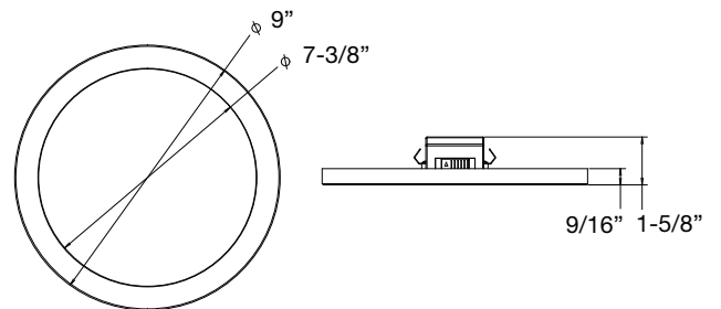
SLMFT9/9CCTS/DIM010UNV
